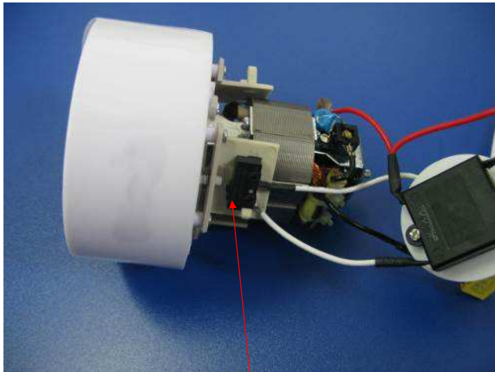
Interlock switch
