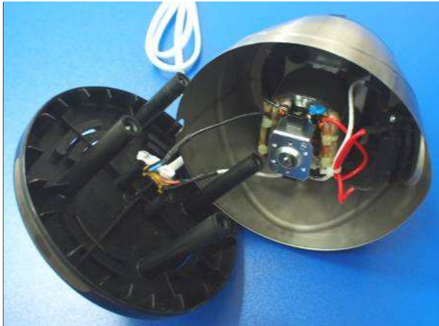
Internal view of model KL-217F
