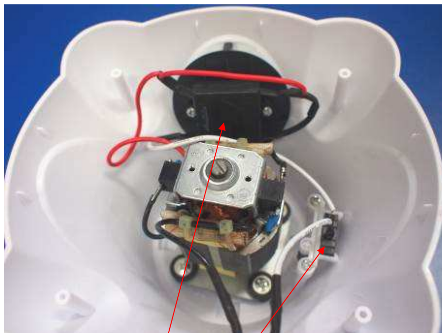
Main switch
