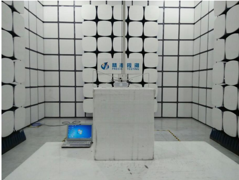
Spurious Emissions 30-1000MHz
