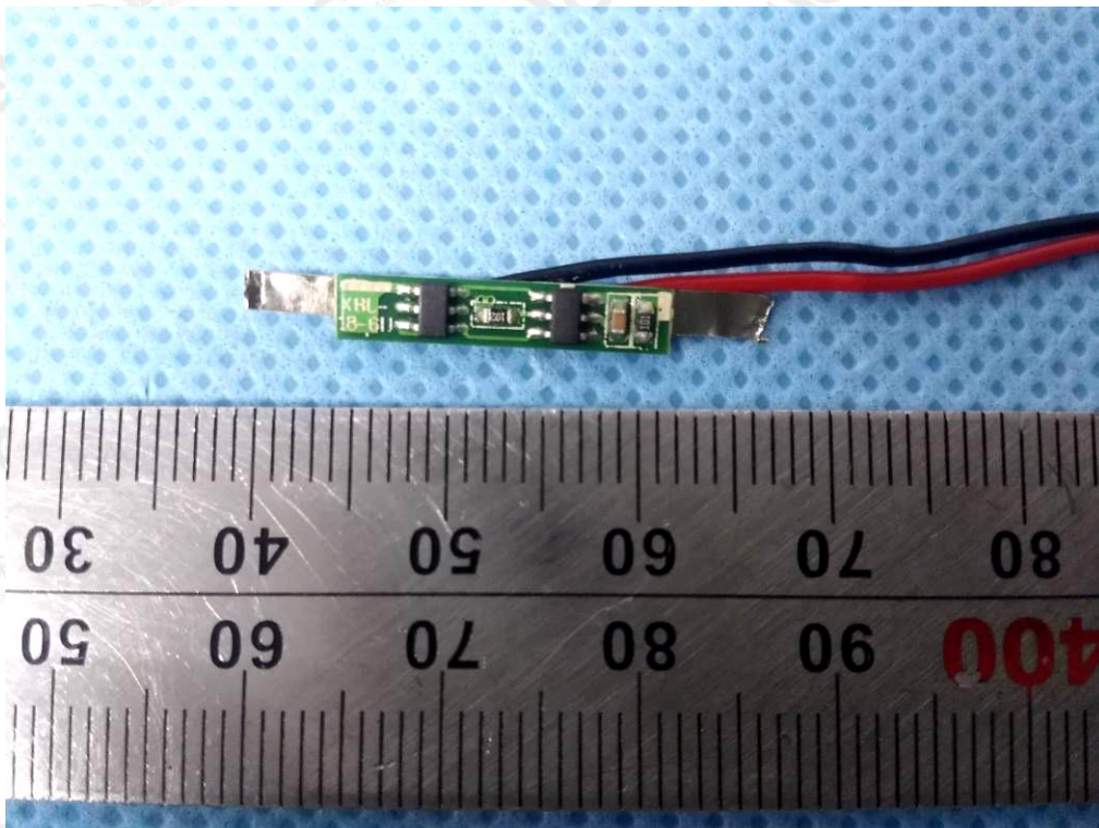
Fig.8 – protect board of battery
