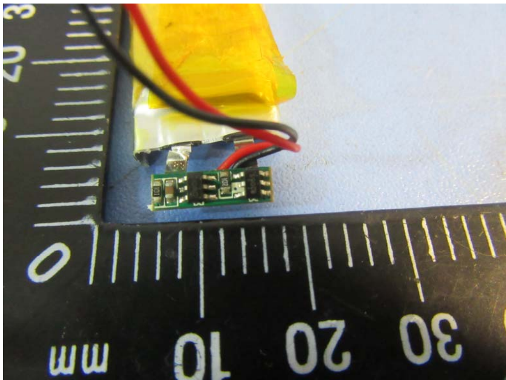
Figure 8. Battery view
