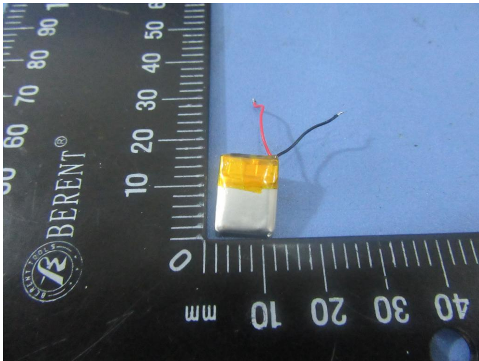
Figure 9. Battery view
