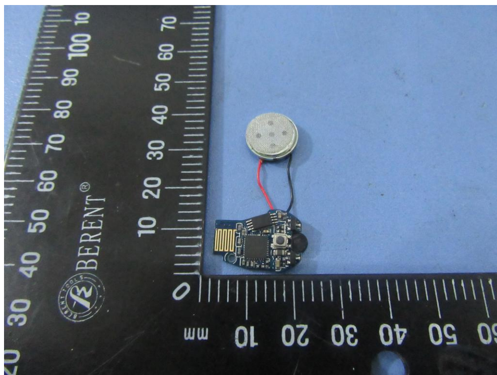
Figure 7. PCB top view
