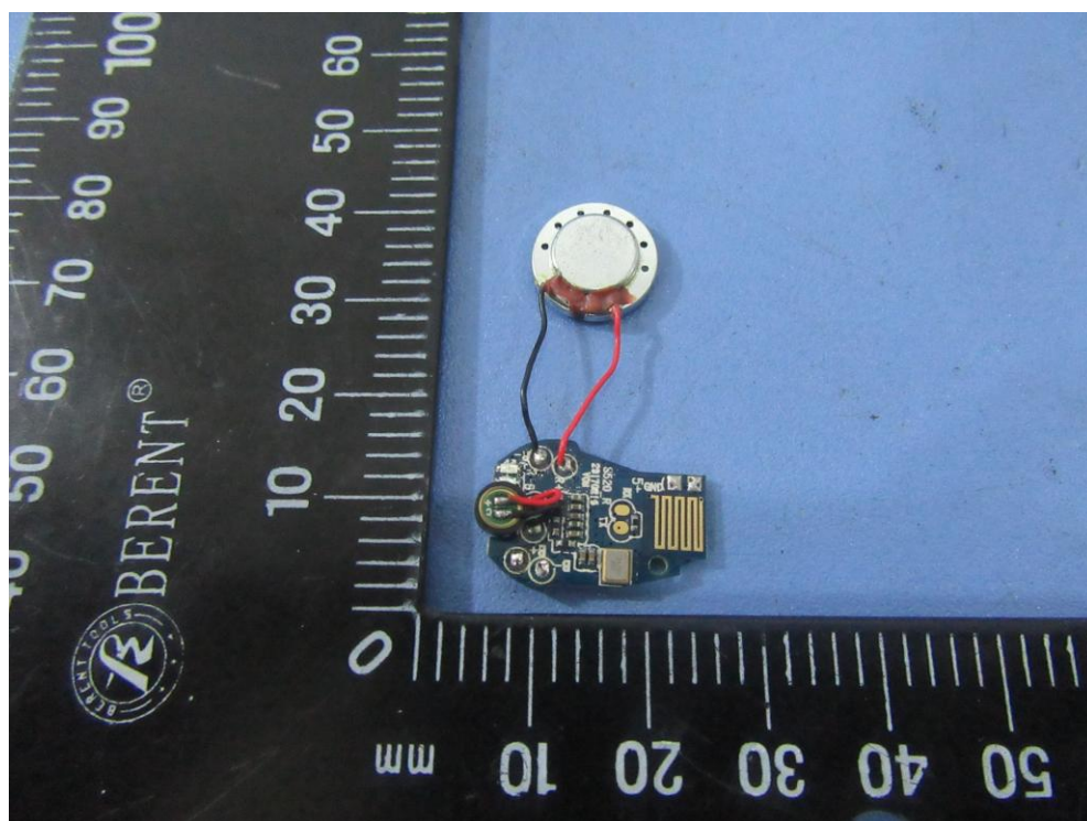
Figure 8. PCB bottom view
