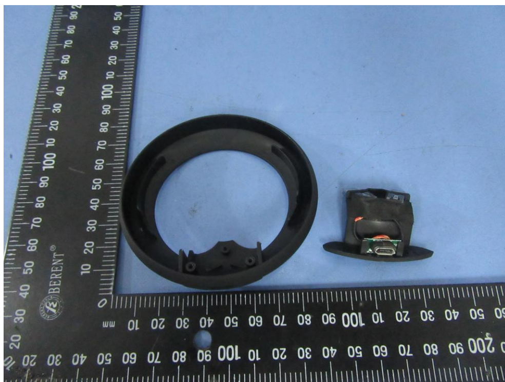
Fig10. Internal view
