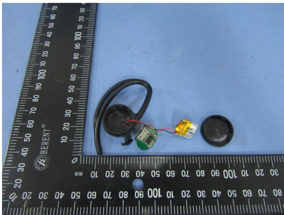
Fig6.internal view
