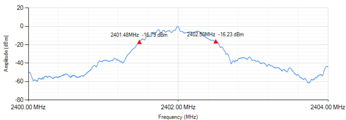
Occupied Channel Bandwidth
