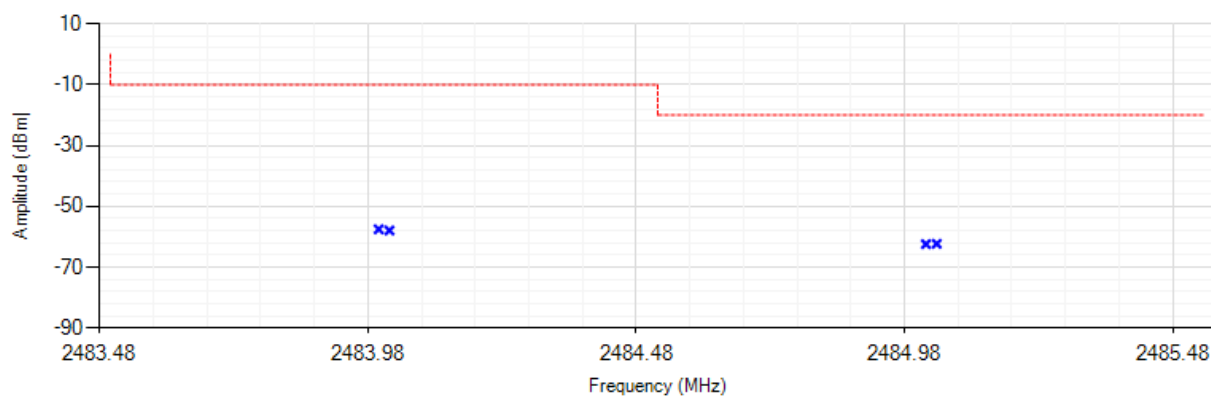
Transmitter unwanted emissions in the out-of-band domain
