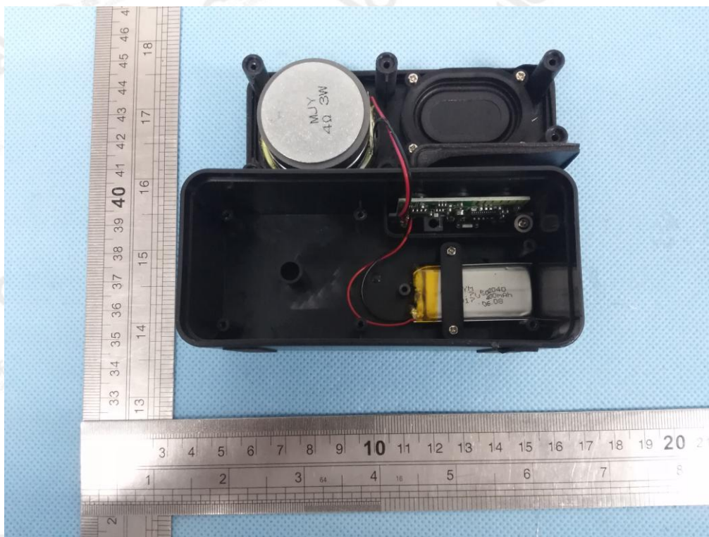
Fig.4- Uncover view
