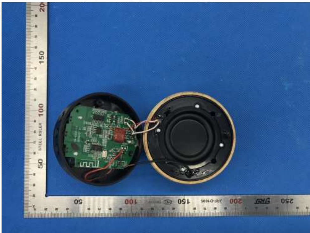
Fig.4 –uncover view
