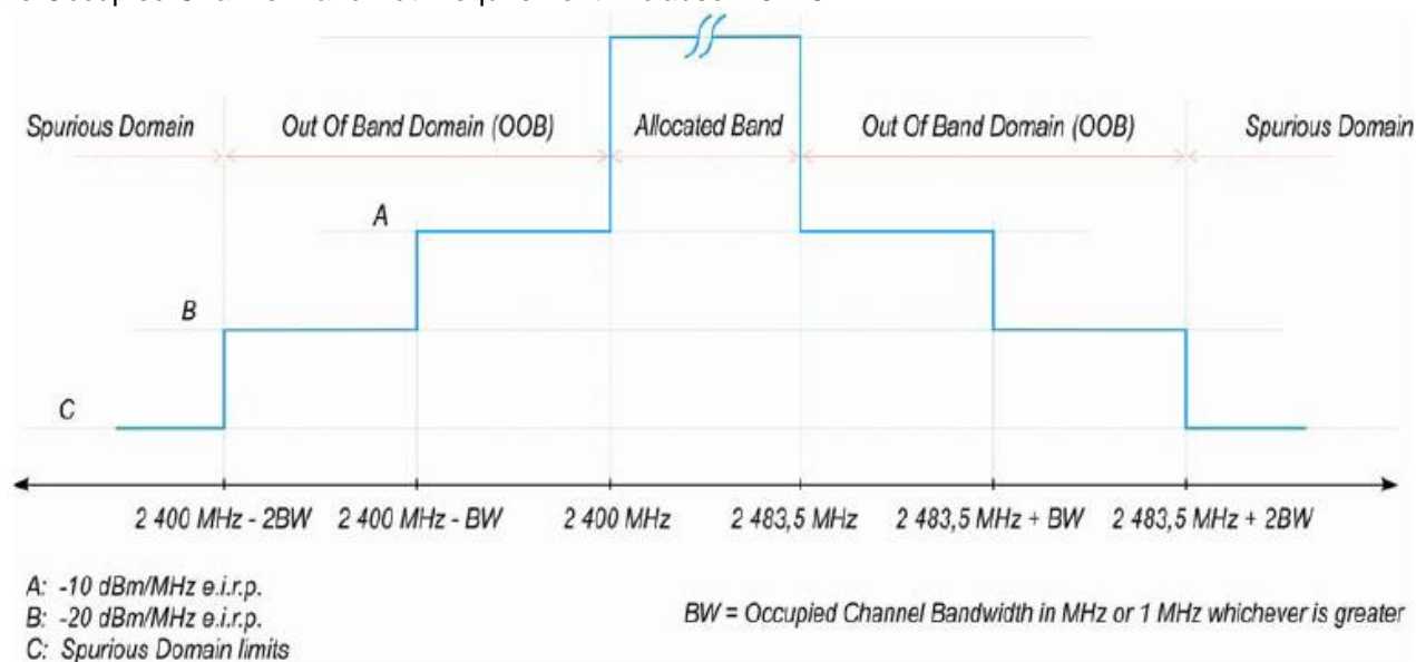
Figure 1: Transmit mask
