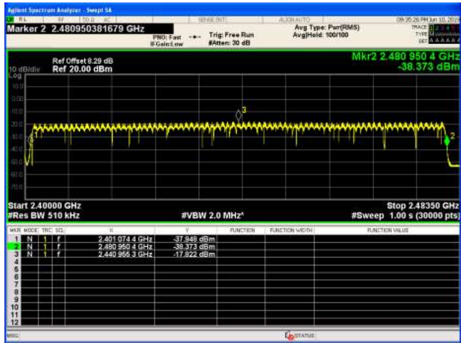
Hopping Sequence_TNVN_GFSK
