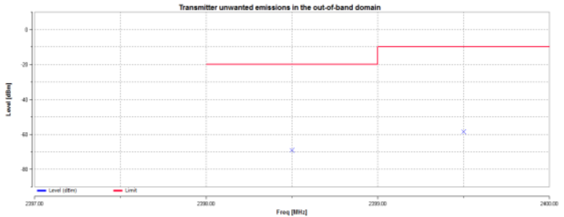
Transmitter unwanted emissions in the OOB domain_TNVN_GFSK_2402_2400MHz-2BW to 2400MHz
