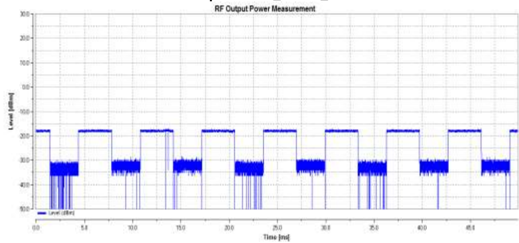
RF Output Power_THVN_GFSK
