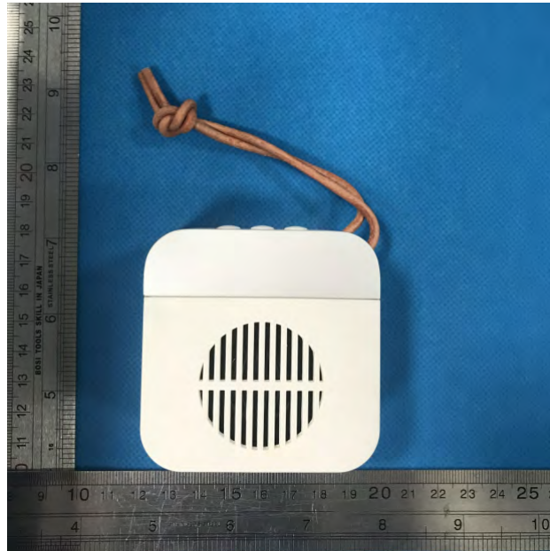
Photo 1 Appearance of EUT
