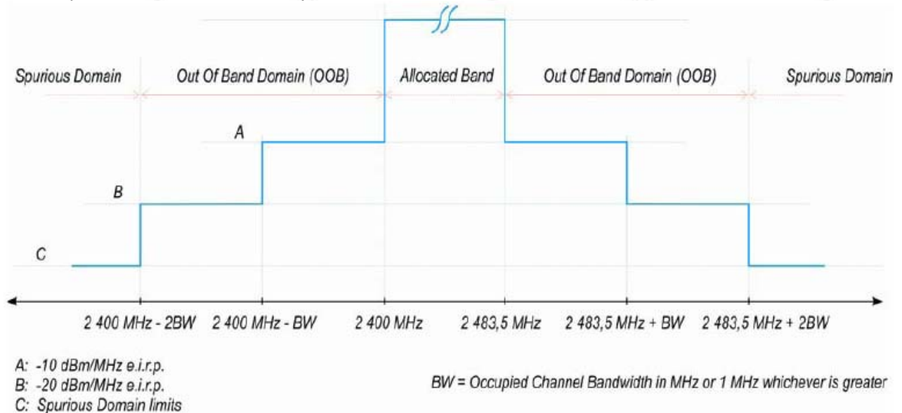
Figure 1: Transmit mask
