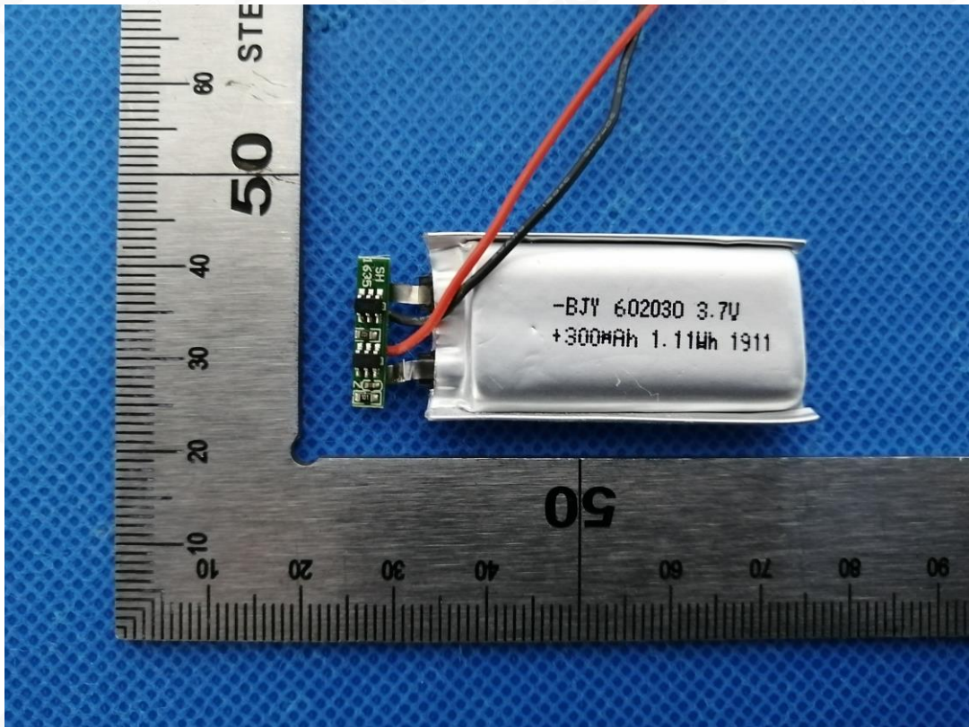
Fig.9 – Battery protection circuit
