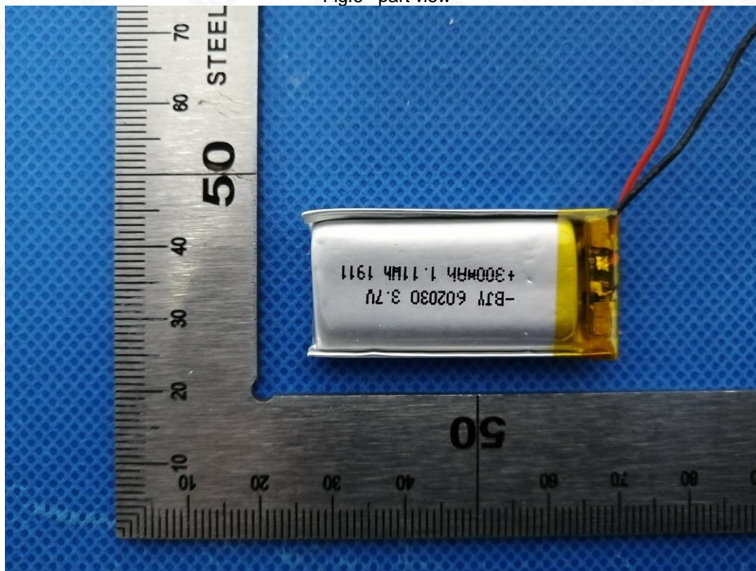
Fig.7 – Battery
