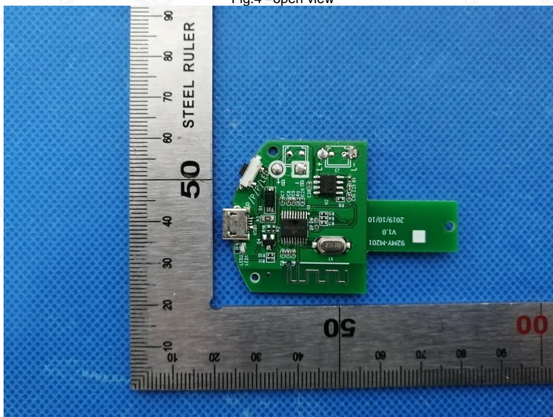
Fig.5 –part view
