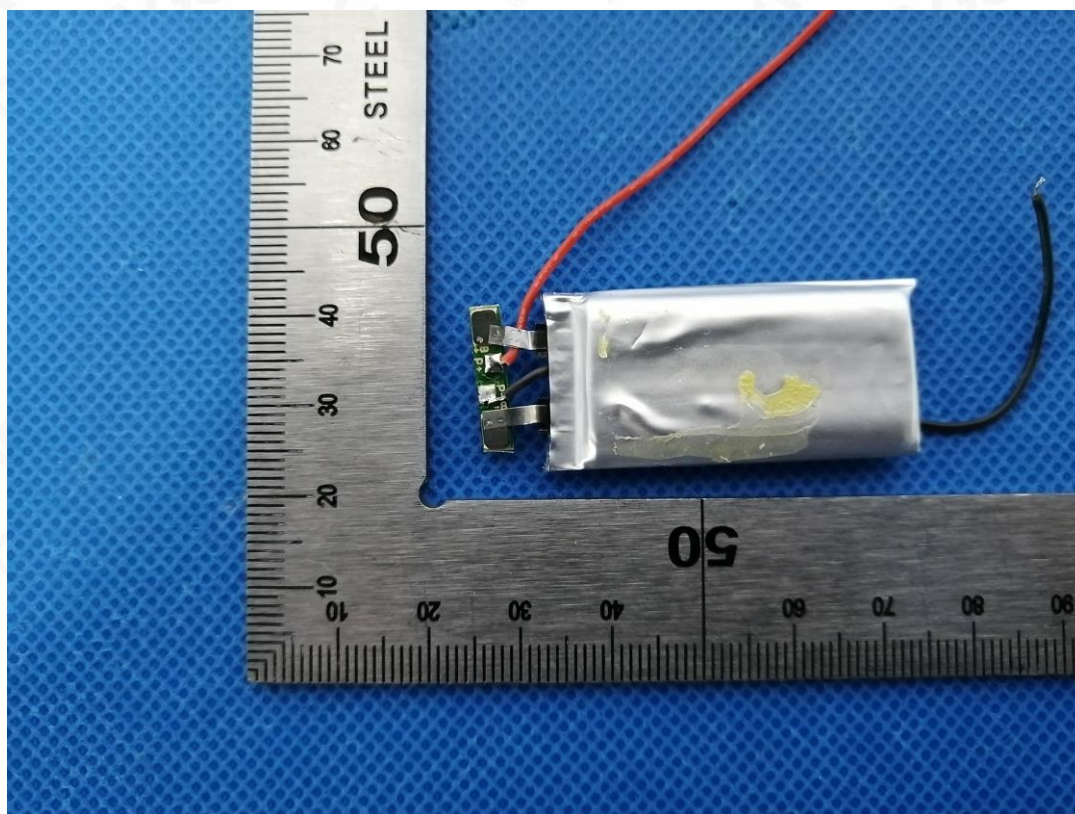
Fig.7 – Battery
