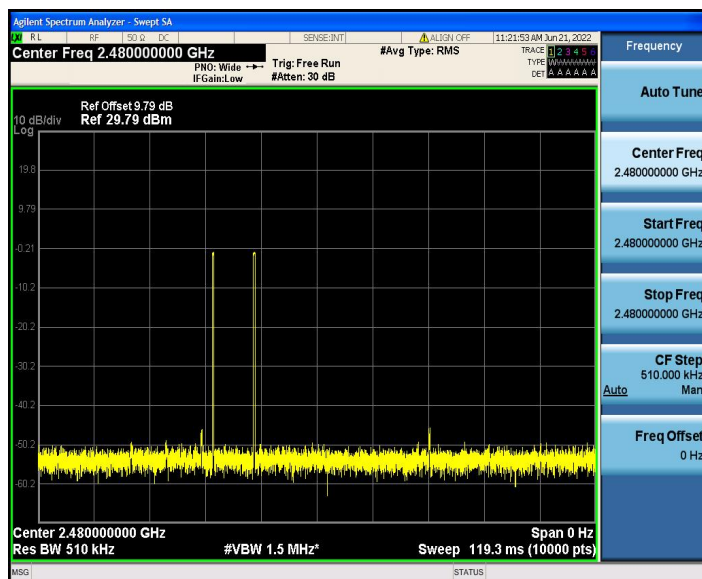
GFSK-DH3: 2480 MHz
