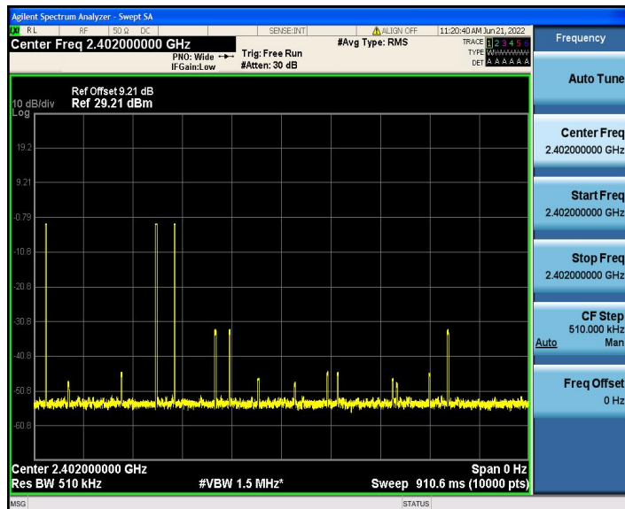
GFSK-DH5: 2402 MHz
