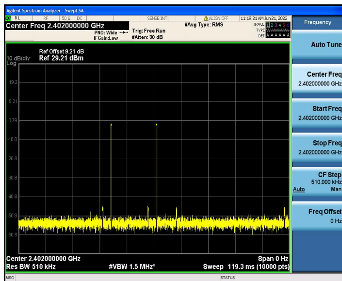
GFSK-DH3: 2402 MHz
