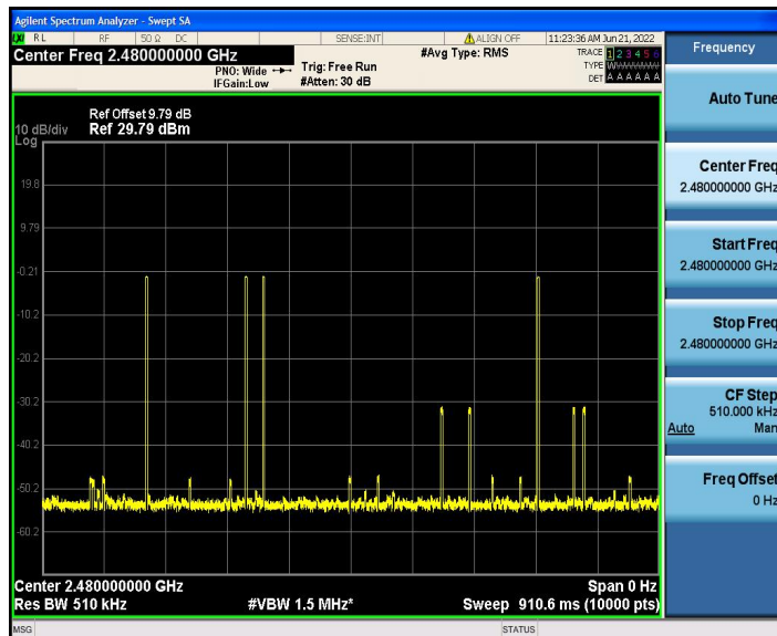
GFSK-DH5: 2480 MHz
