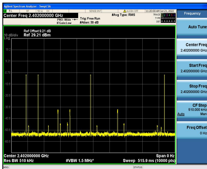
GFSK-DH5: 2402 MHz
